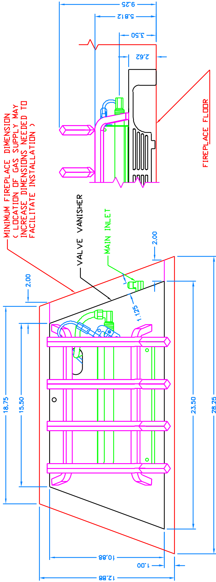
TOP VIEW
